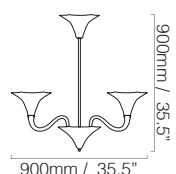
3 Lights
