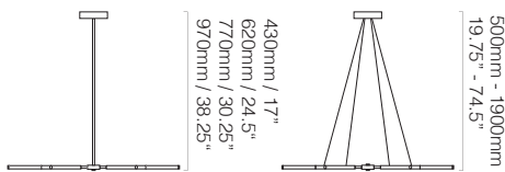
Fixed Stem
